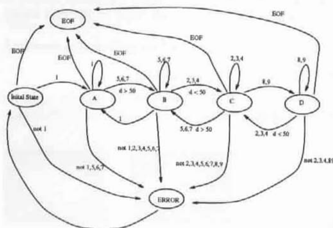
FIG. 2. State machine used in test.
